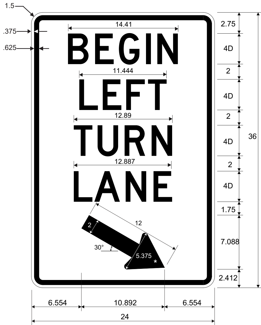
R3-20L BEGIN LEFT TURN LANE (Arrow)
