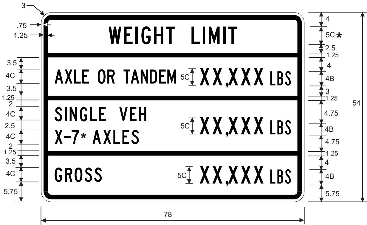
R12-8hT WEIGHT LIMIT
