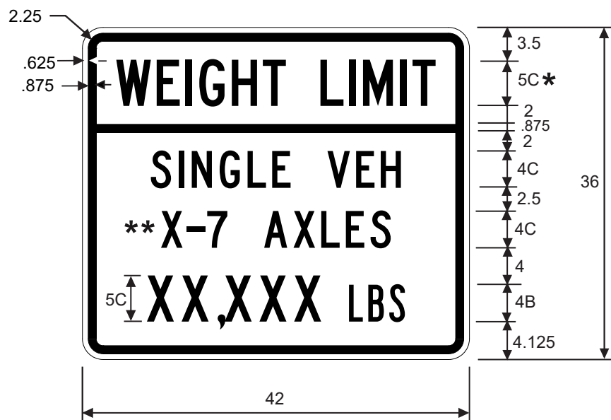
R12-8mT WEIGHT LIMIT
