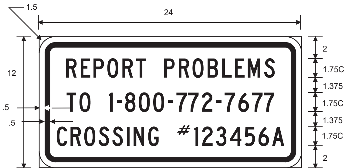
R15-4 REPORT PROBLEMS TO (Phone number) CROSSING
