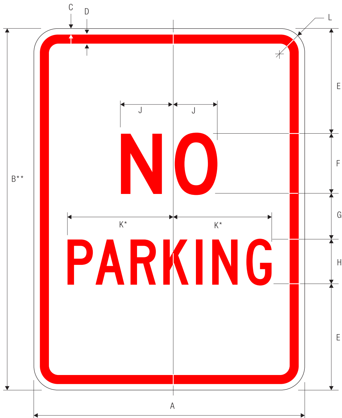
R8-3a NO PARKING
