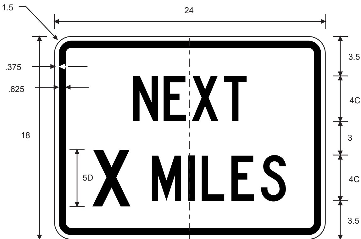
R20-1TP NEXT X MILES (Plaque)
