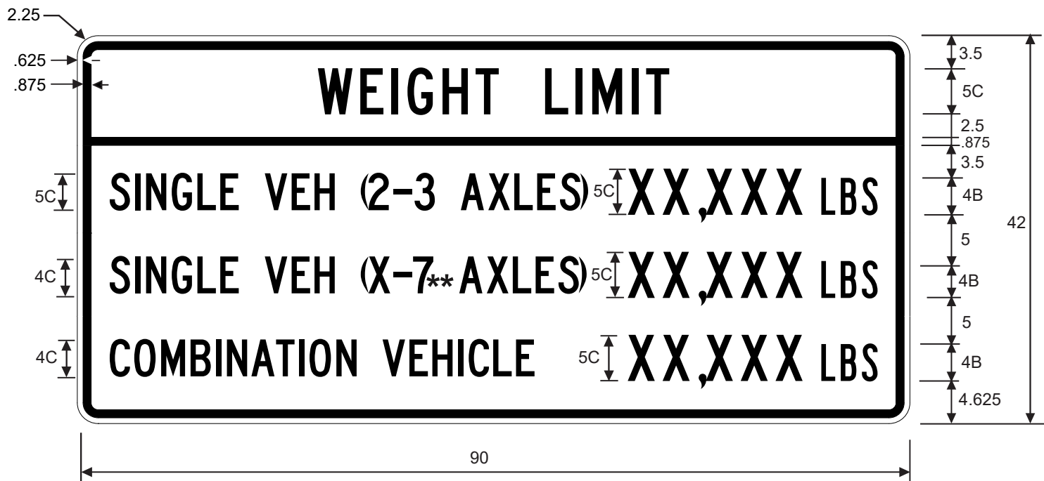
R12-8kT WEIGHT LIMIT
