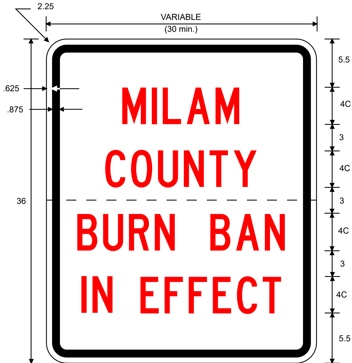
R19-10bT (Folding Sign) COUNTY BURN BAN IN EFFECT
