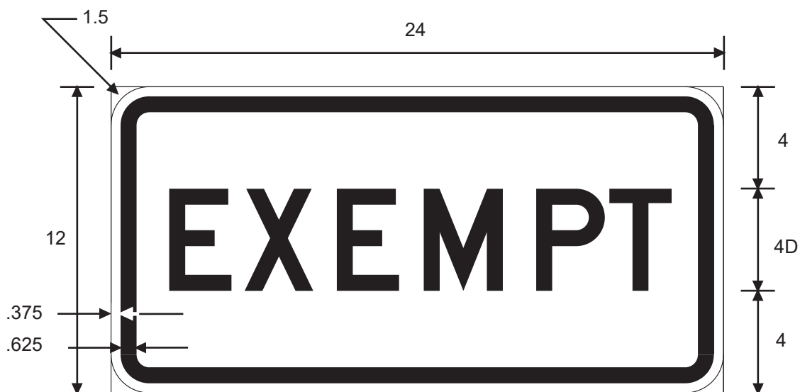
R15-3P EXEMPT (Plaque)
