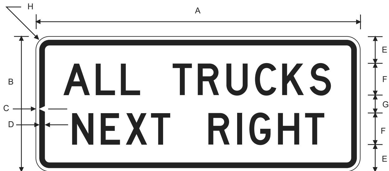
R13-1TPR ALL TRUCKS NEXT RIGHT
