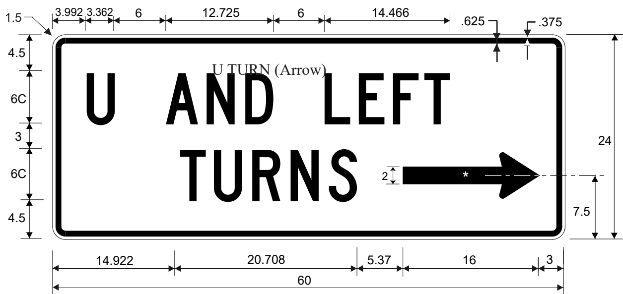
R3-25a U TURN AND LEFT TURNS (Arrow)
