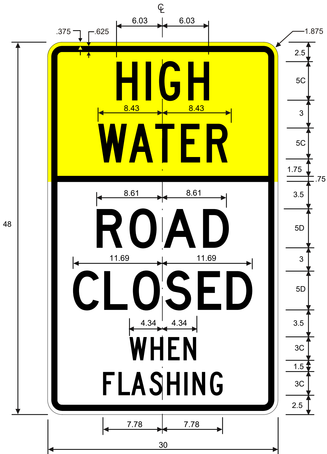
R11-5bT HIGH WATER ROAD CLOSED WHEN FLASHING
