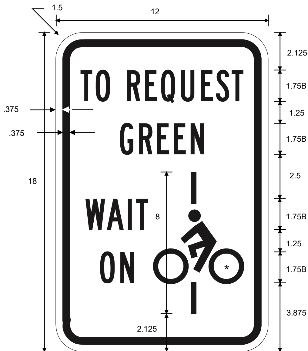
R10-22 TO REQUEST GREEN WAIT ON (Bike symbol)
