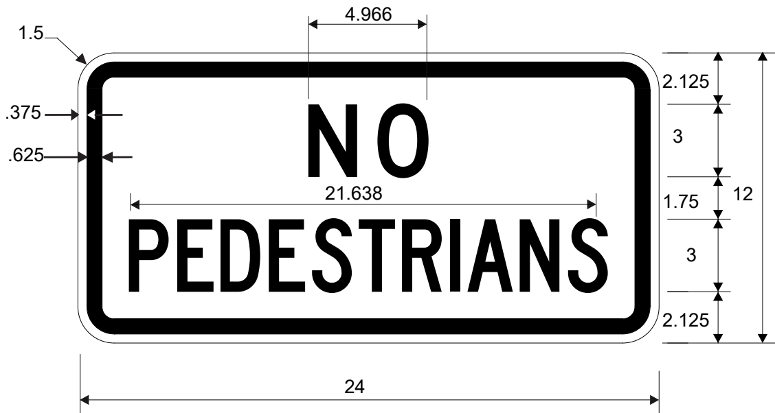
R5-10c NO PEDESTRIANS
