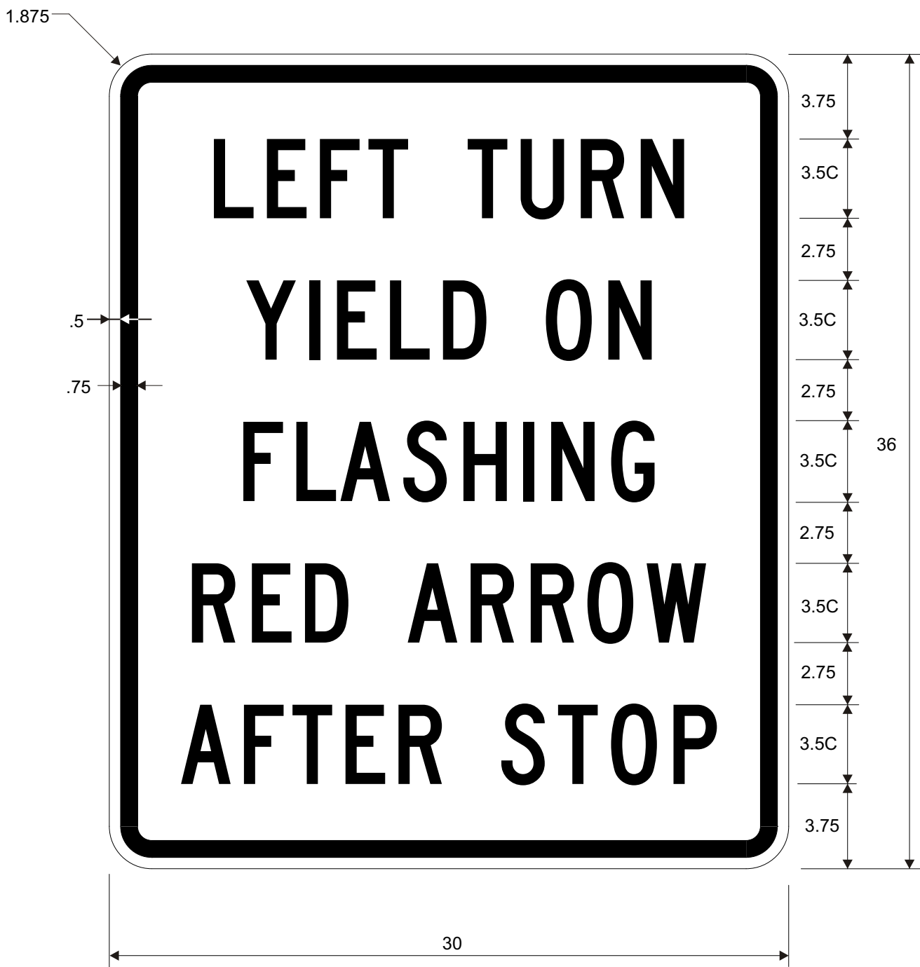
R10-27 LEFT TURN YIELD ON FLASHING RED ARROW AFTER STOP
