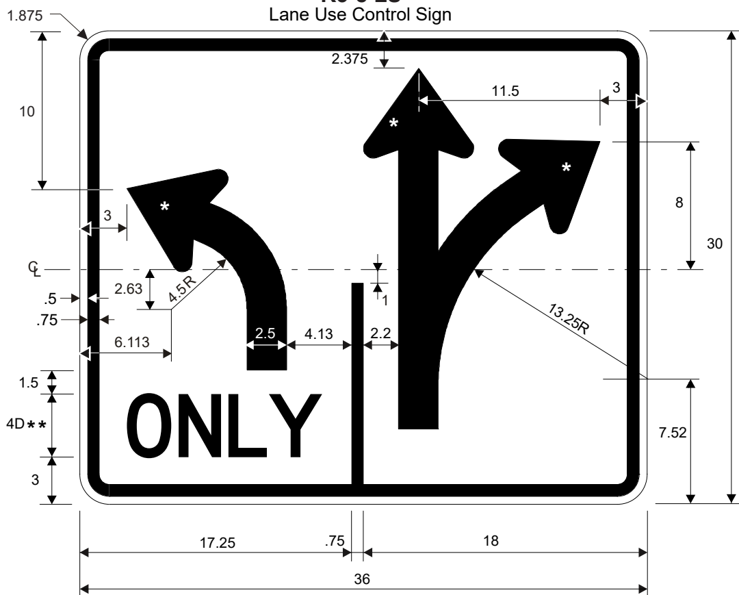
R3-8 LK Lane Use Control Sign
