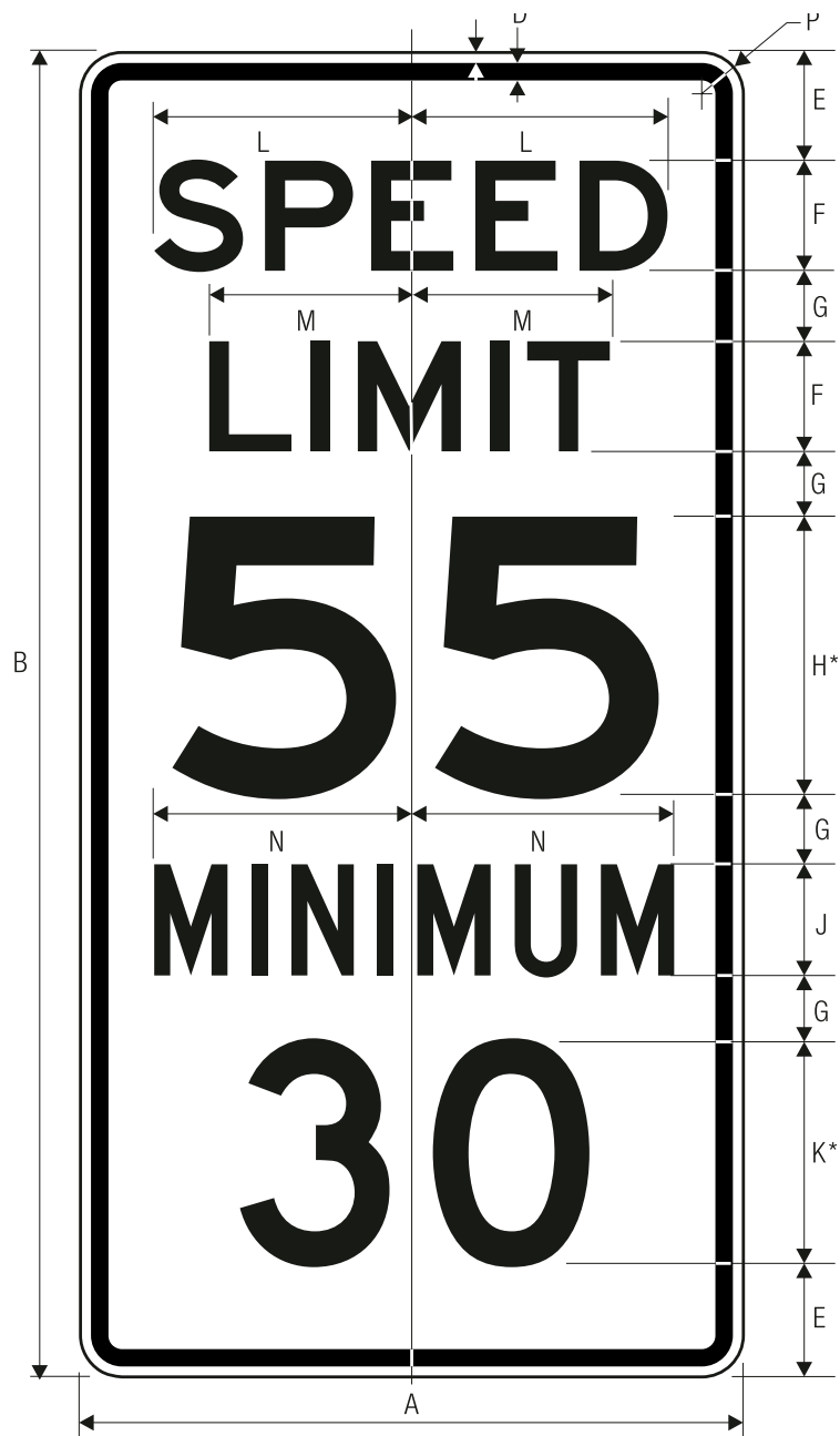
R2-4a COMBINED SPEED LIMIT
