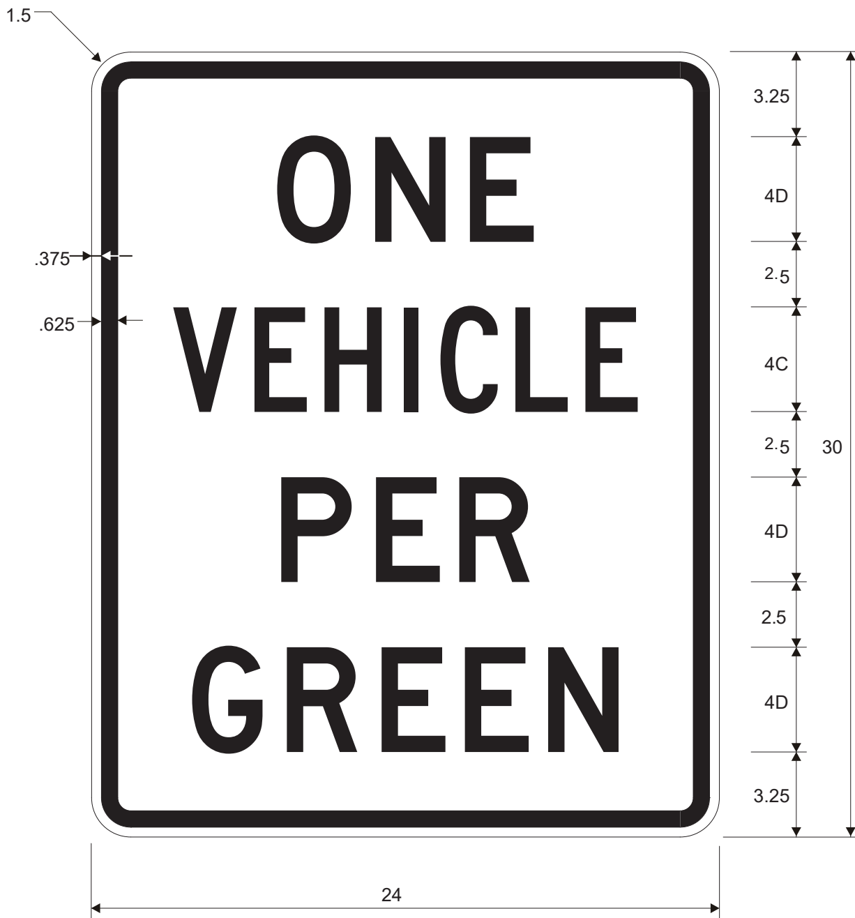
R10-28 ONE VEHICLE PER GREEN
