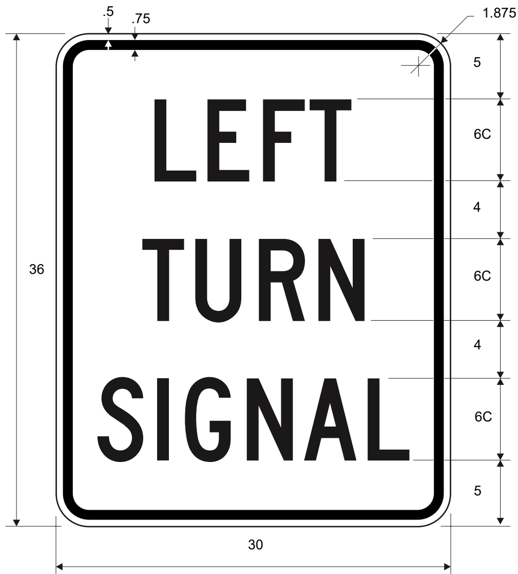
R10-10L LEFT/RIGHT TURN SIGNAL
