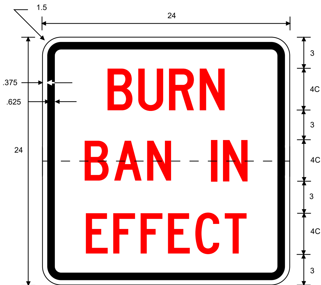
R19-10aT (Folding Sign) BURN BAN IN EFFECT
