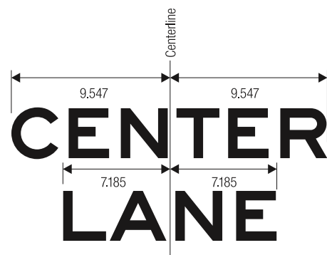
R15-4c LIGHT RAIL ONLY CENTER LANE
