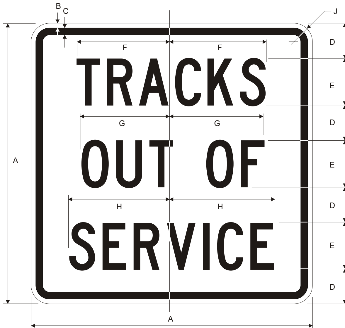
R8-9 TRACKS OUT OF SERVICE
