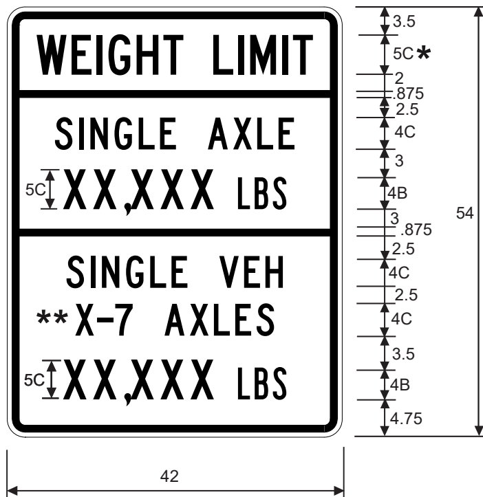
R12-8dT WEIGHT LIMIT
