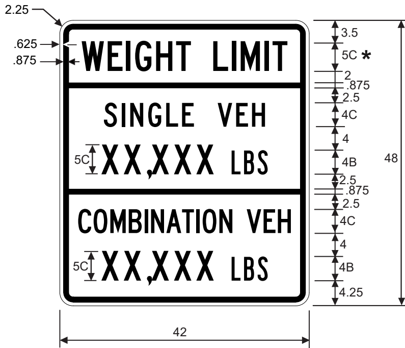
R12-8cT WEIGHT LIMIT
