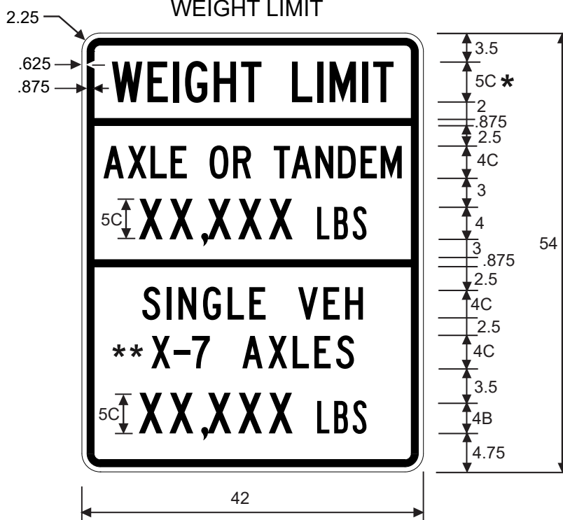
R12-8fT WEIGHT LIMIT
