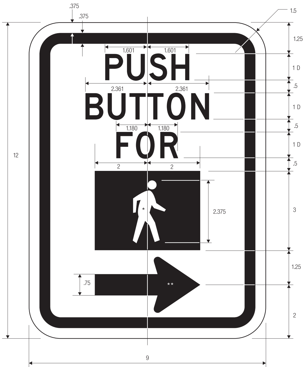
R10-4bR PUSH BUTTON FOR (Symbol)
