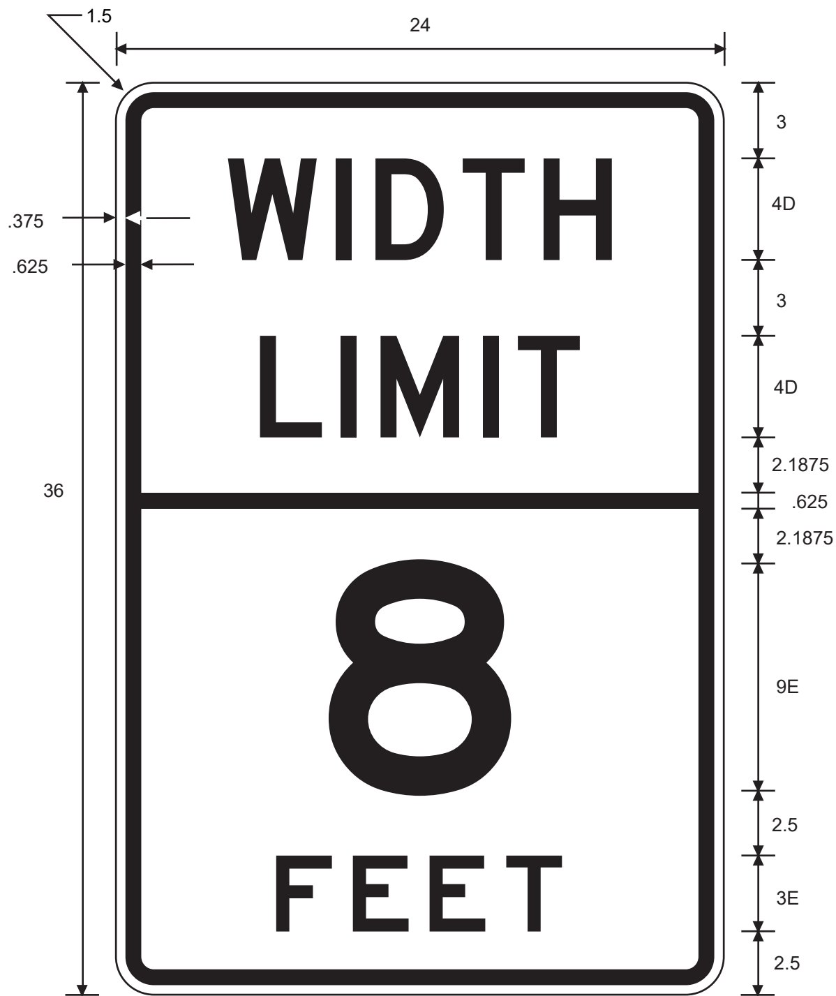
R12-9T WIDTH LIMIT 8 FEET
