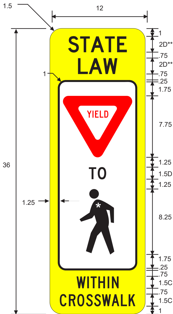
R1-6 IN-STREET PED CROSSING (Ped symbol)
