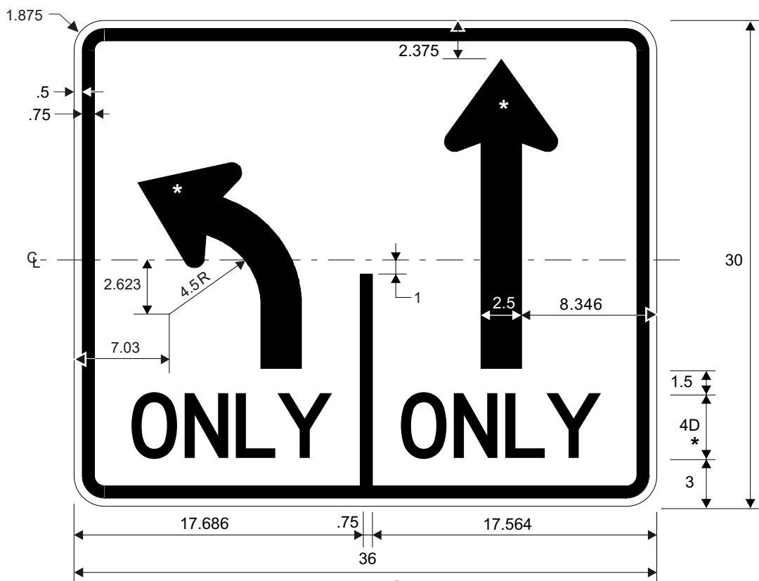
R3-8 LS Lane Use Control Sign
