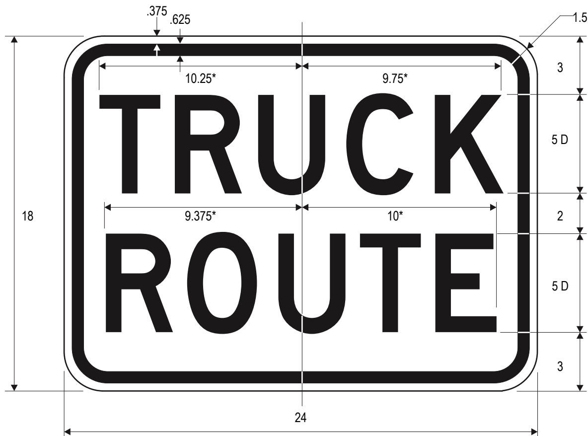
R14-1 TRUCK ROUTE
