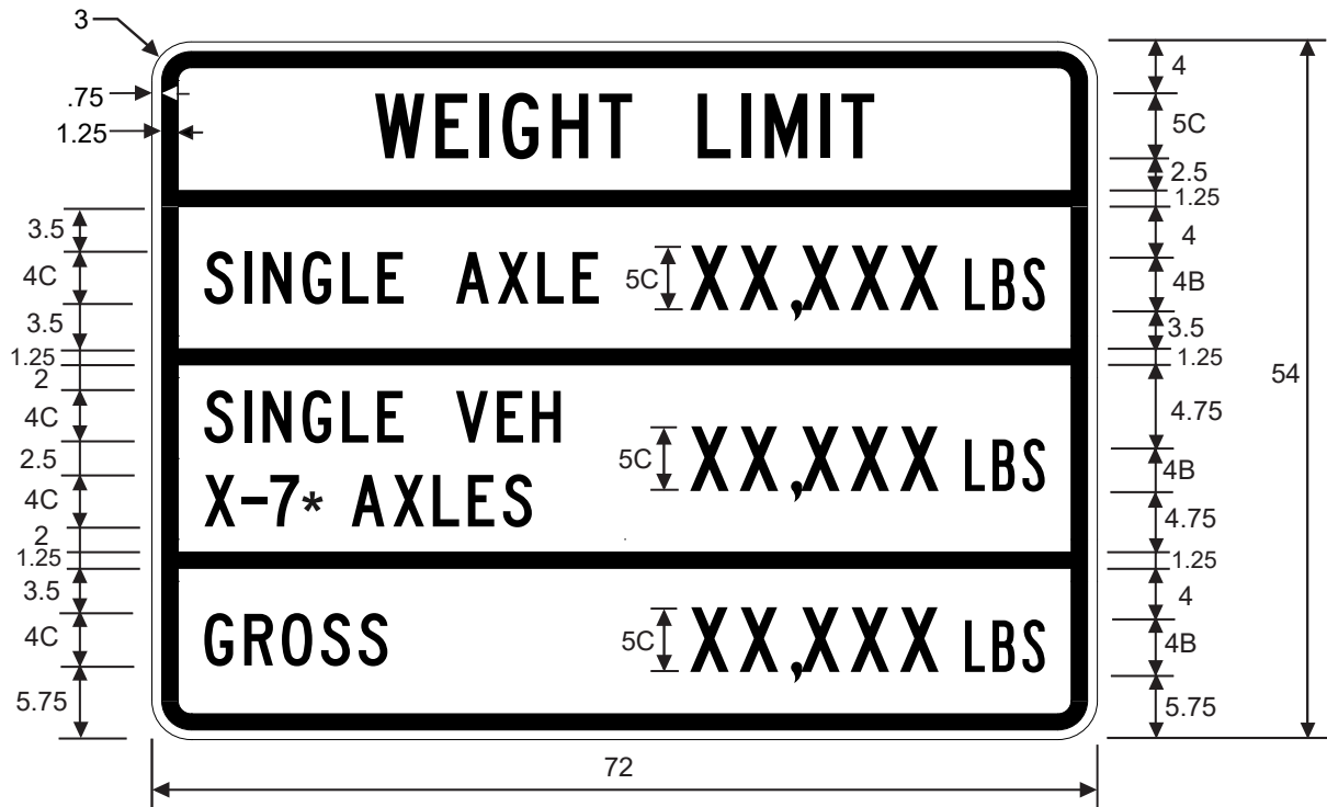
R12-8gT WEIGHT LIMIT
