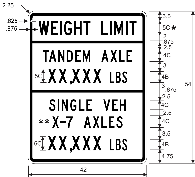
R12-8eT WEIGHT LIMIT
