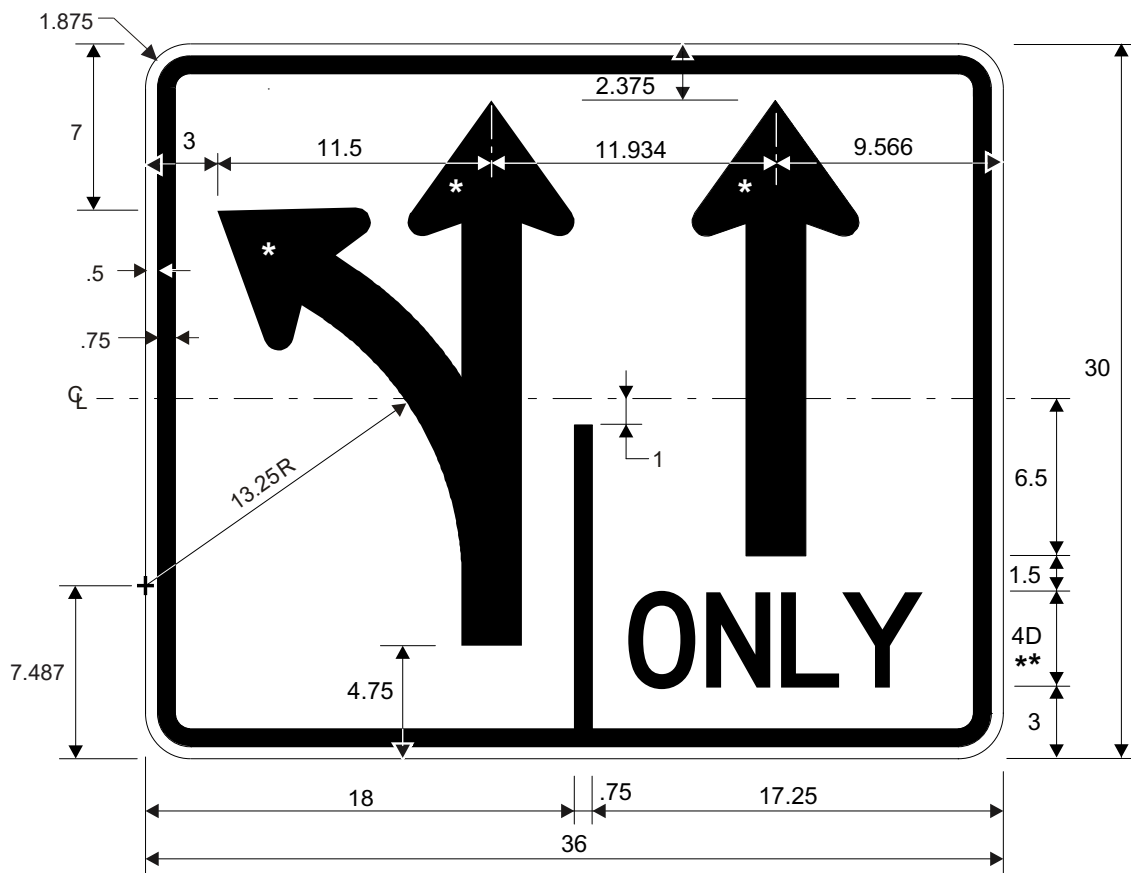
R3-8 MS Lane Use Control Sign
