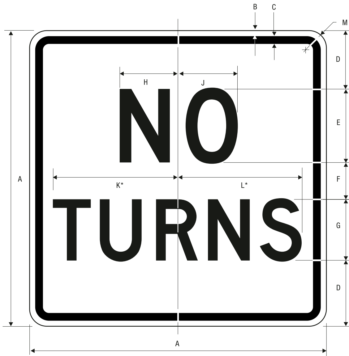
R3-3 NO TURNS
