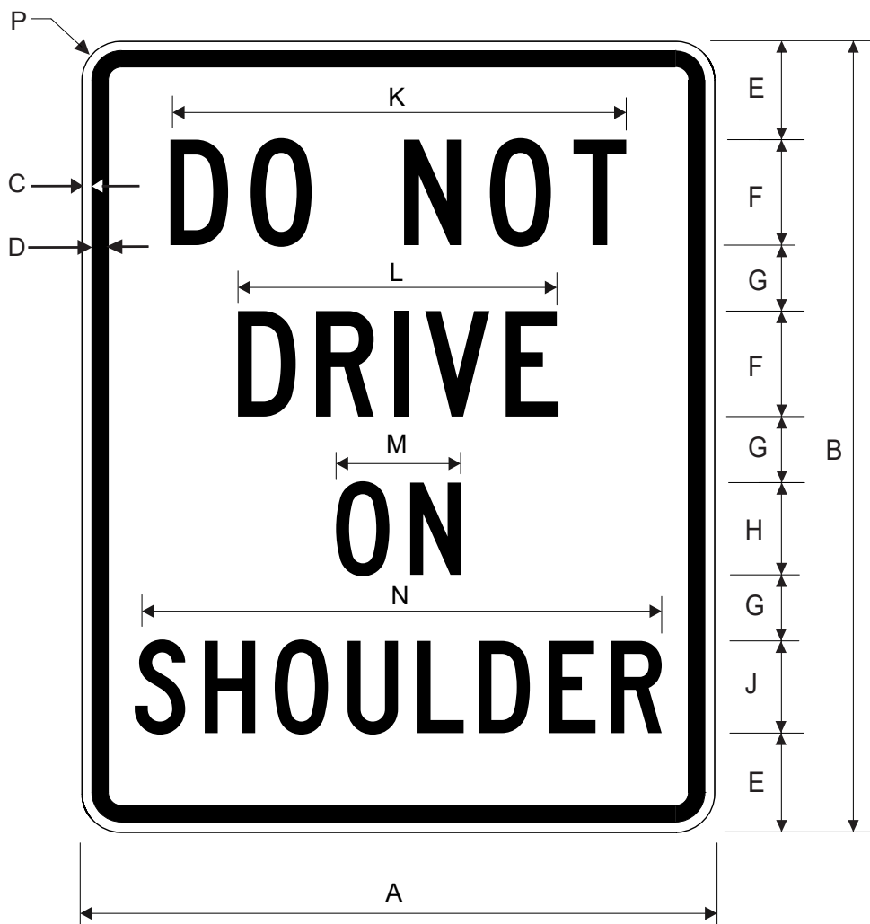
R4-17 DO NOT DRIVE ON SHOULDER
