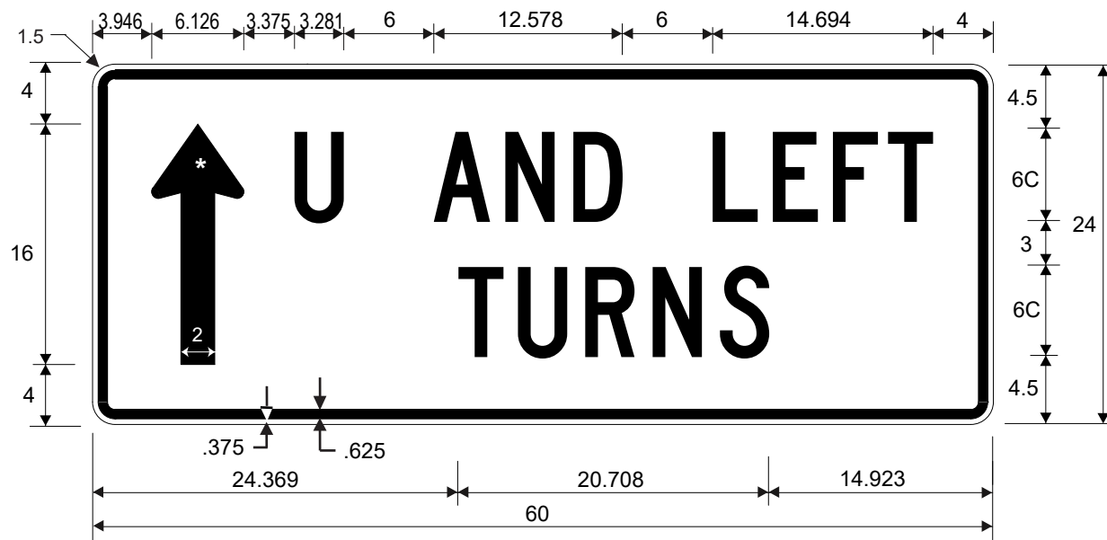
R3-26 U TURN AND LEFT TURNS (Up Arrow)
