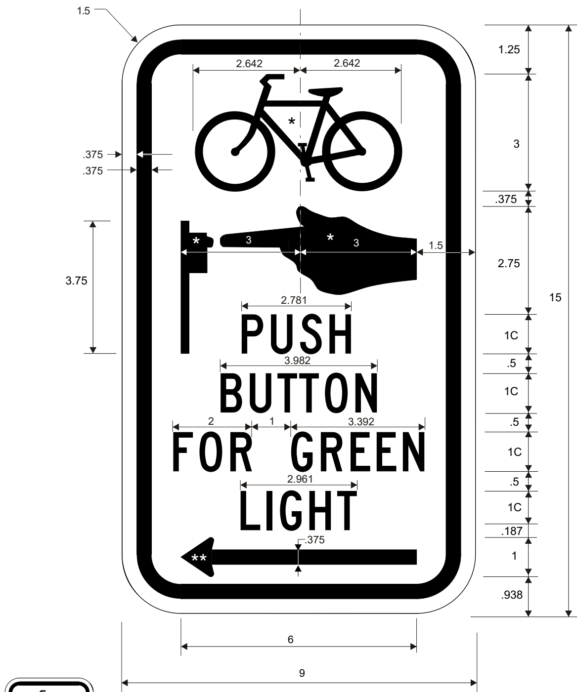
R10-26L PUSH BUTTON FOR GREEN LIGHT (Symbols/Arrow)
