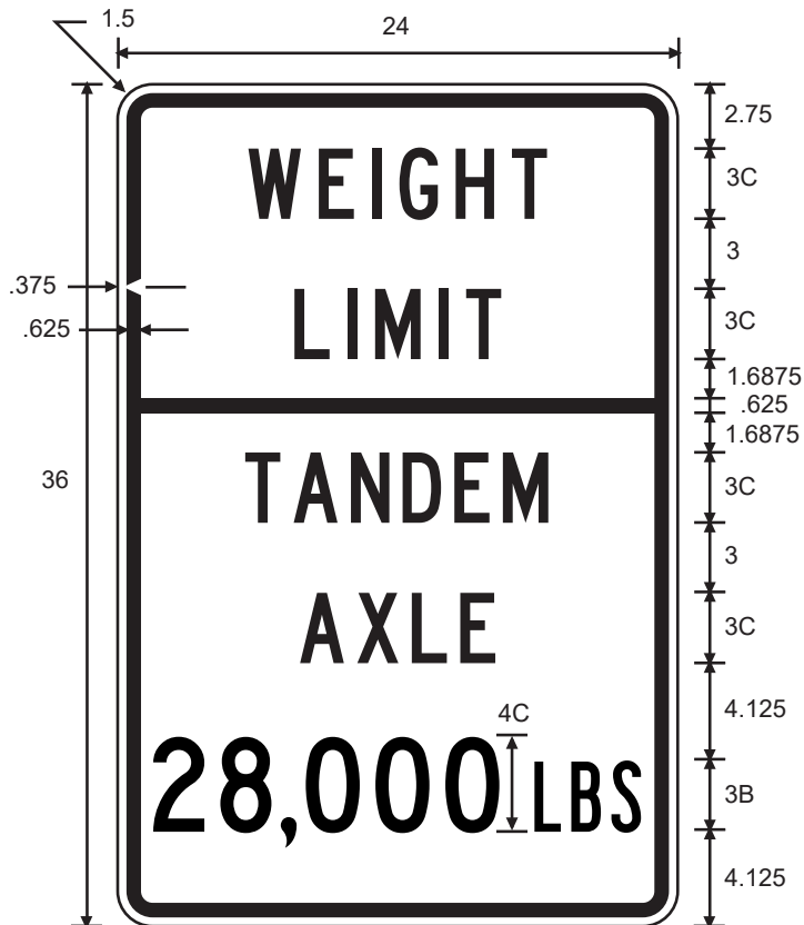
R12-2cT WEIGHT LIMIT
