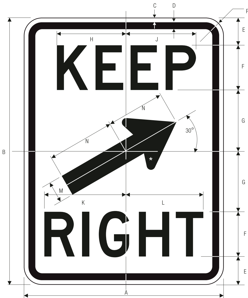
R4-7b KEEP RIGHT (30° Arrow)
