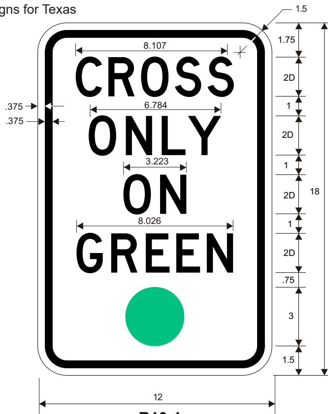
R10-1 CROSS ONLY ON GREEN (Green ball)
